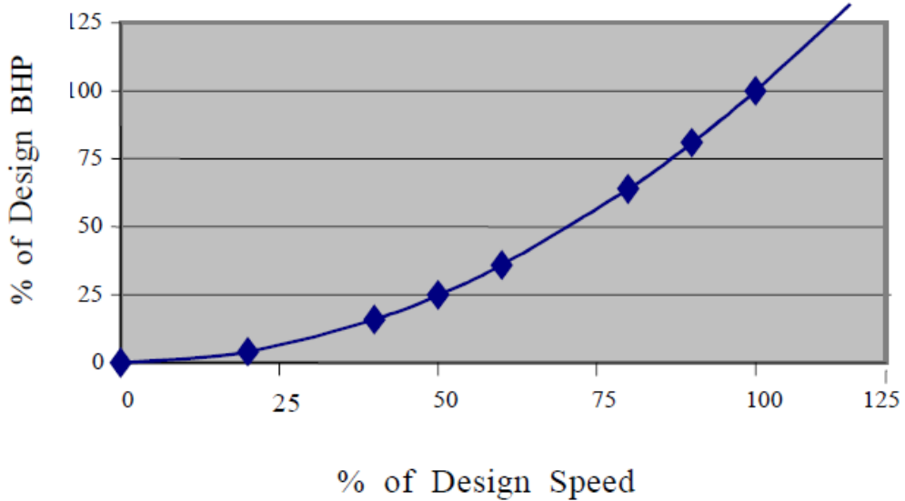
Motor Power vs Motor Speed
