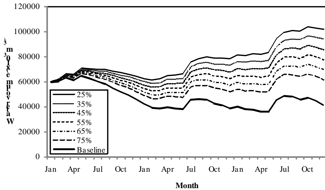
Figure 9: Sensitivity results for the volume of water pumped to coastal cities tests.
