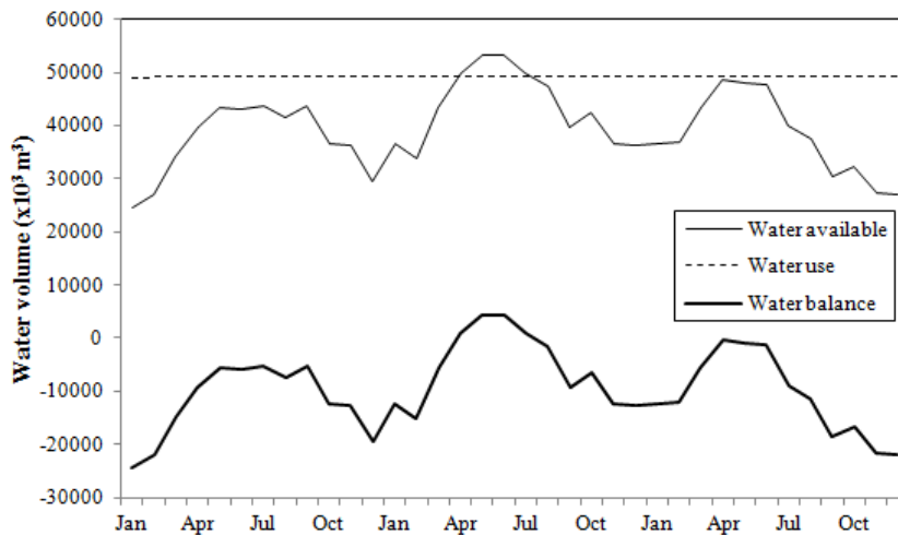
Figure 14: Baseline mode results for the Rosetta case study.
