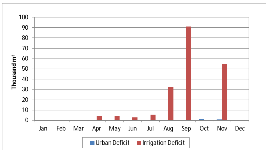
Figure 26: Water deficit in the urban and agricultural sectors for the 2010 baseline
