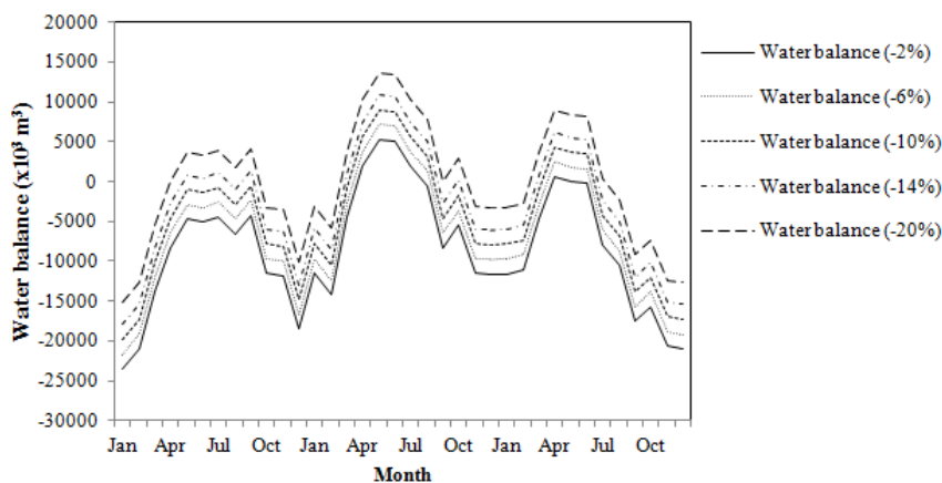
Figure 16: Results of the land loss sensitivity tests.
