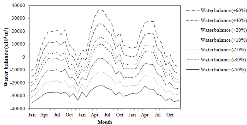
Figure 15: Results of the canal inflow sensitivity tests.
