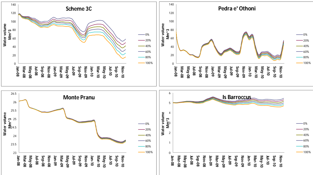
Figure 38: Sensitivity test for domestic demand
