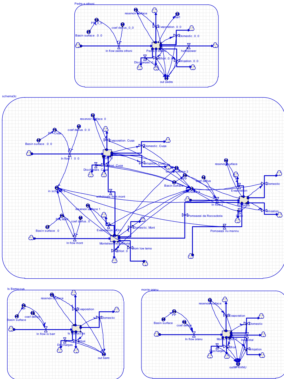
Figure 34: The developed SDM for the Sardinia case study.
