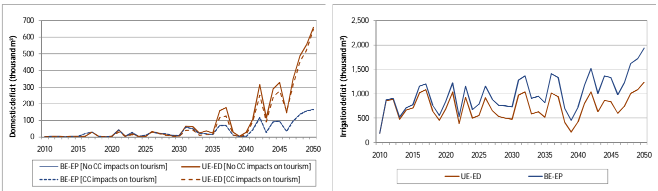
(a) (b) Figure 30: Domestic and irrigation deficits for the BE-EP and UE-ED scenarios for 2010-2050
