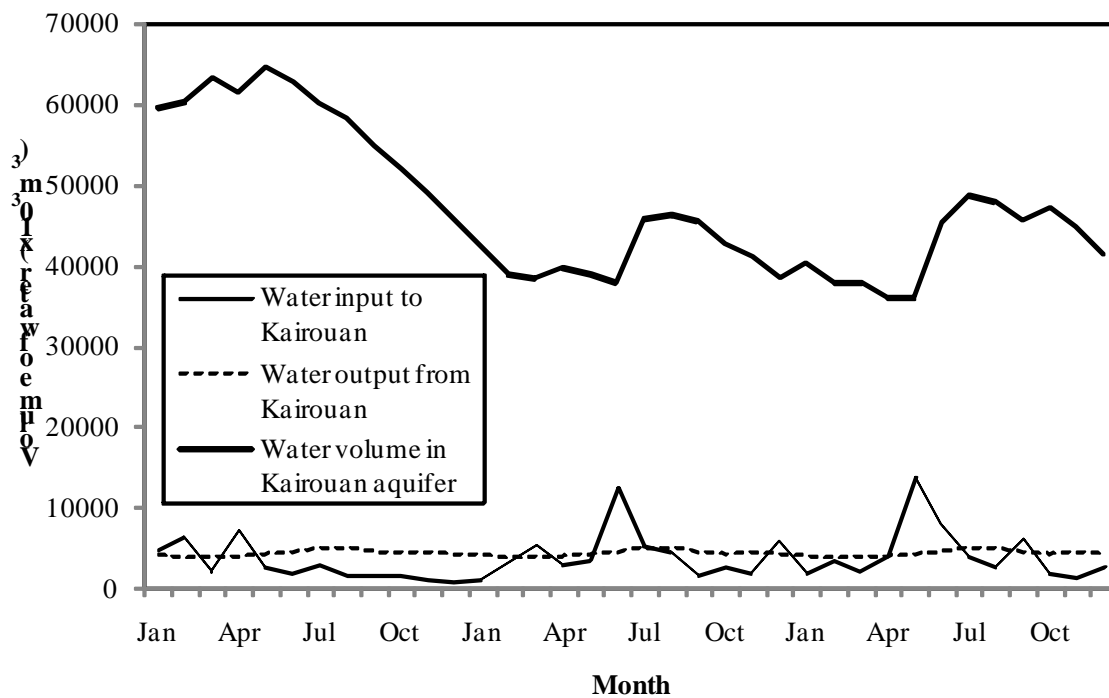
Figure 6: Baseline results for the Kairouan aquifer case study.
